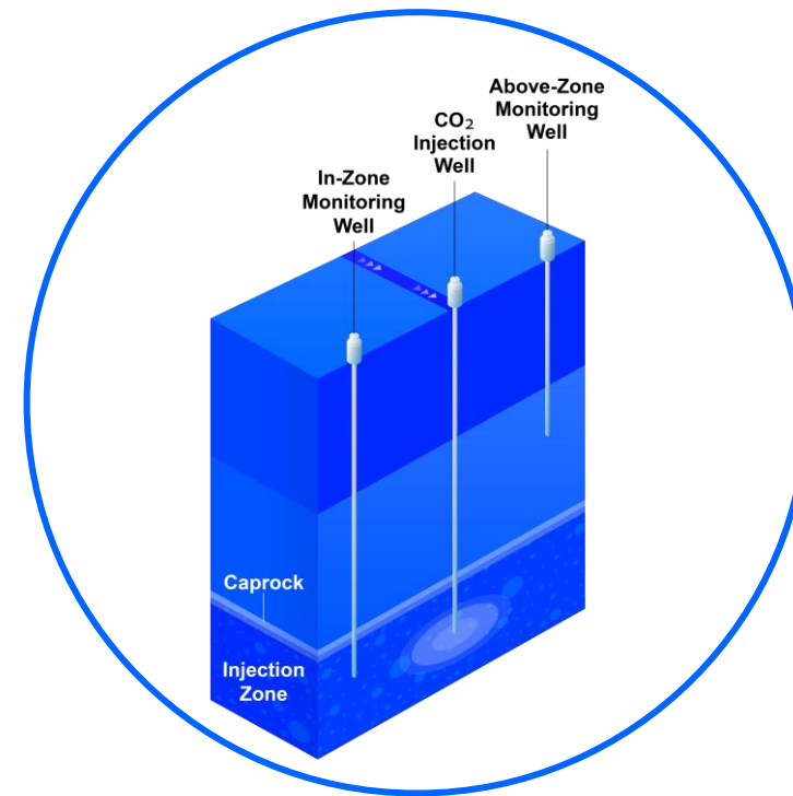
Illustrative example of a CO 2 geologic storage well (not to scale). (Credit: 1PointFive.com)
